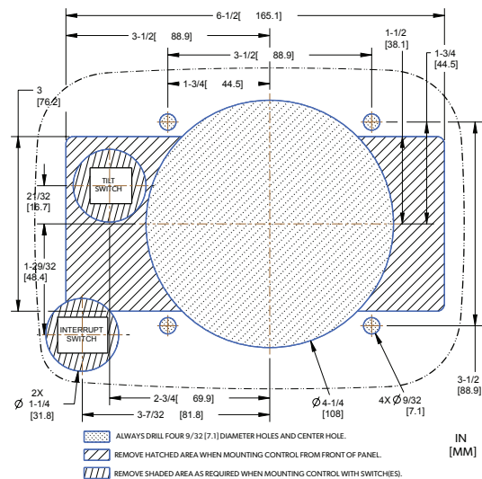
CHX8051P Hole Cutout
